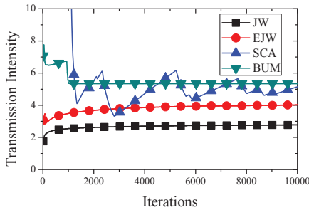
Fig. 1. Intensity traces for the star interference graph with 5 links (i.e., one link interferes with other 4 links which do not interfere with each other). Note that EJW and JW are increasing until 10000 slots.
